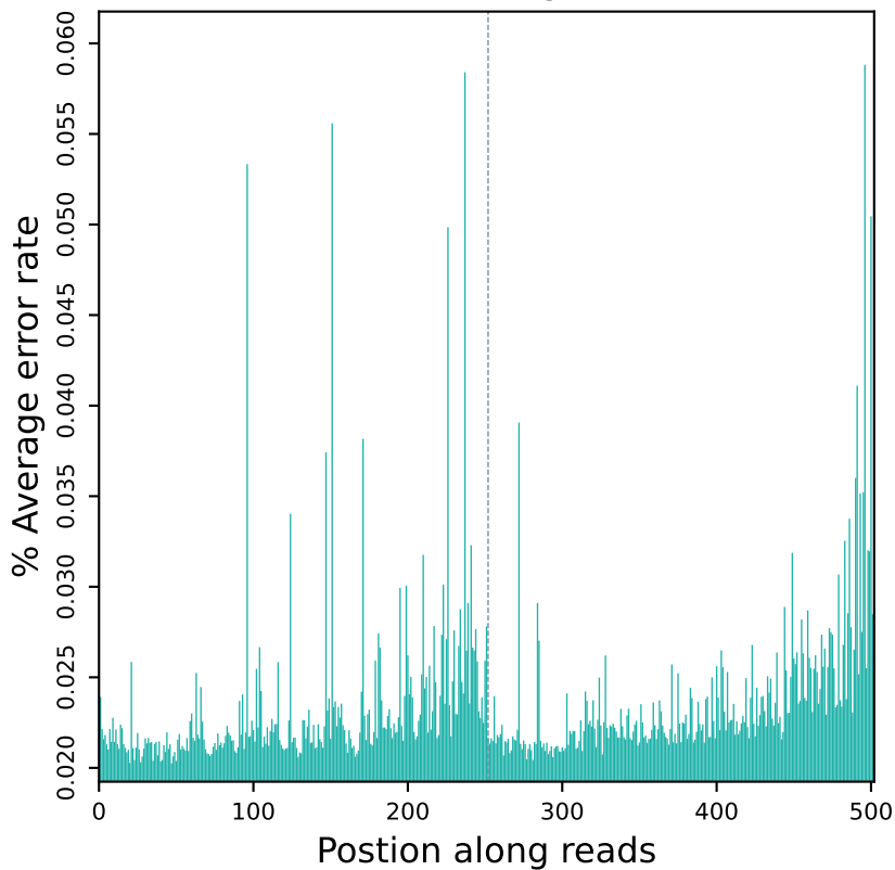
Error rate distribution along reads (R10207)
